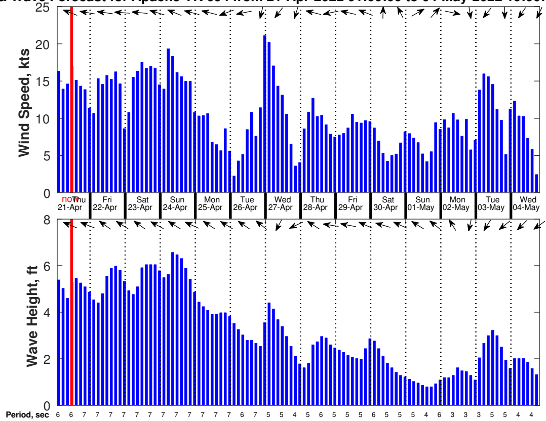
Wind & Wave Forecast for Apache VK 694 from 21-Apr-2022 01:00:00 to 04-May-2022 19:00:00
