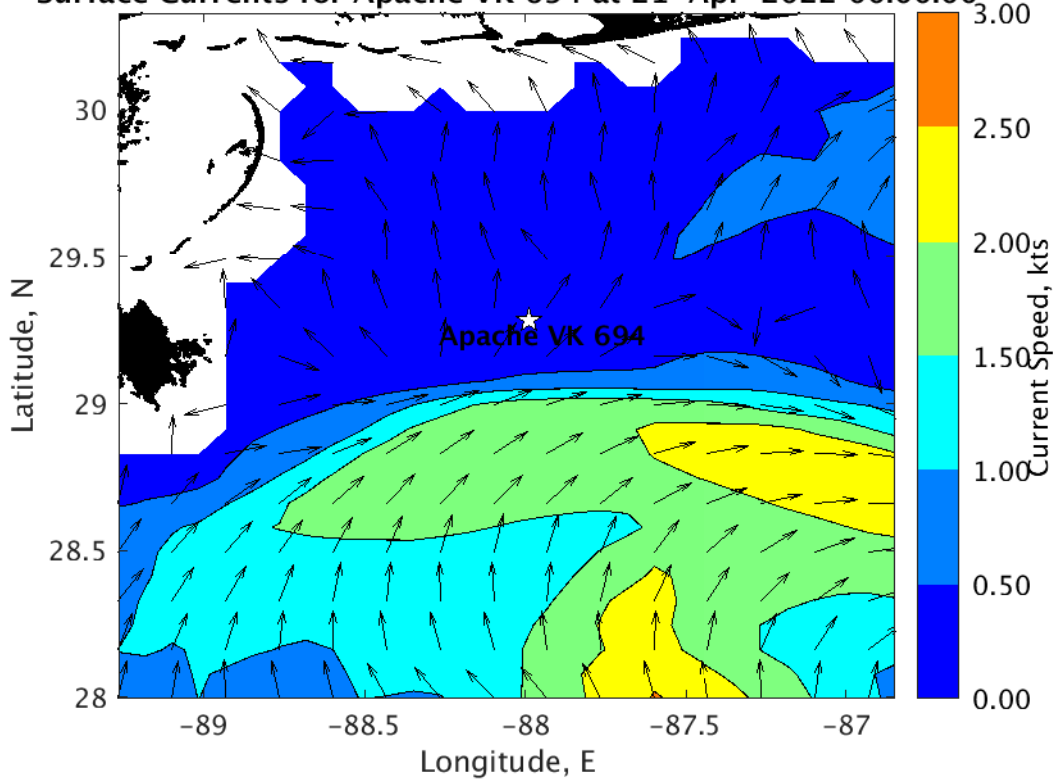
Surface Currents for Apache VK 694 at 21-Apr-2022 00:00:00
