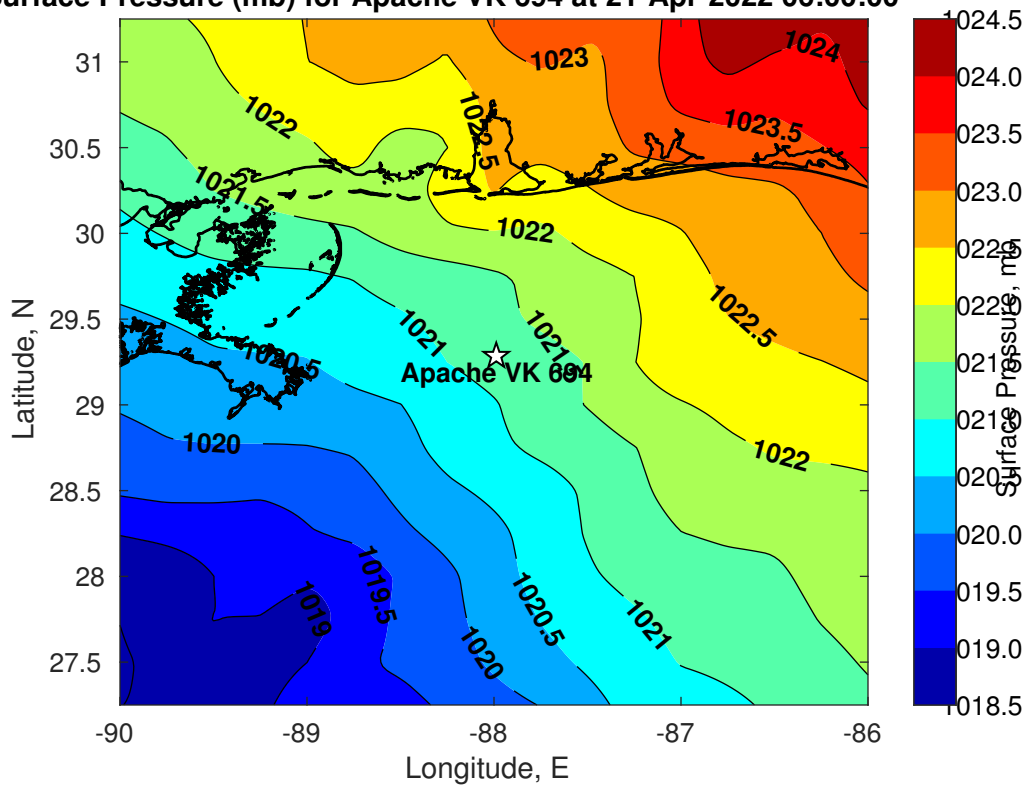
Surface Pressure (mb) for Apache VK 694 at 21-Apr-2022 06:00:00
