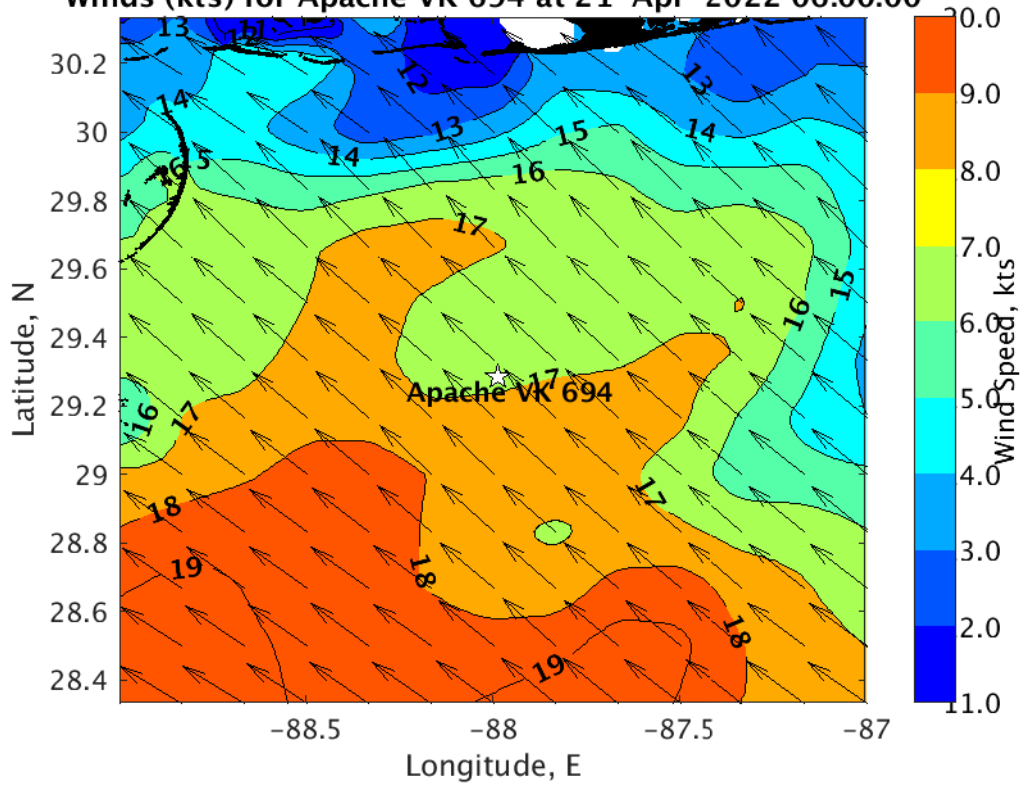
Winds (kts) for Apache VK 694 at 21-Apr-2022 06:00:00
