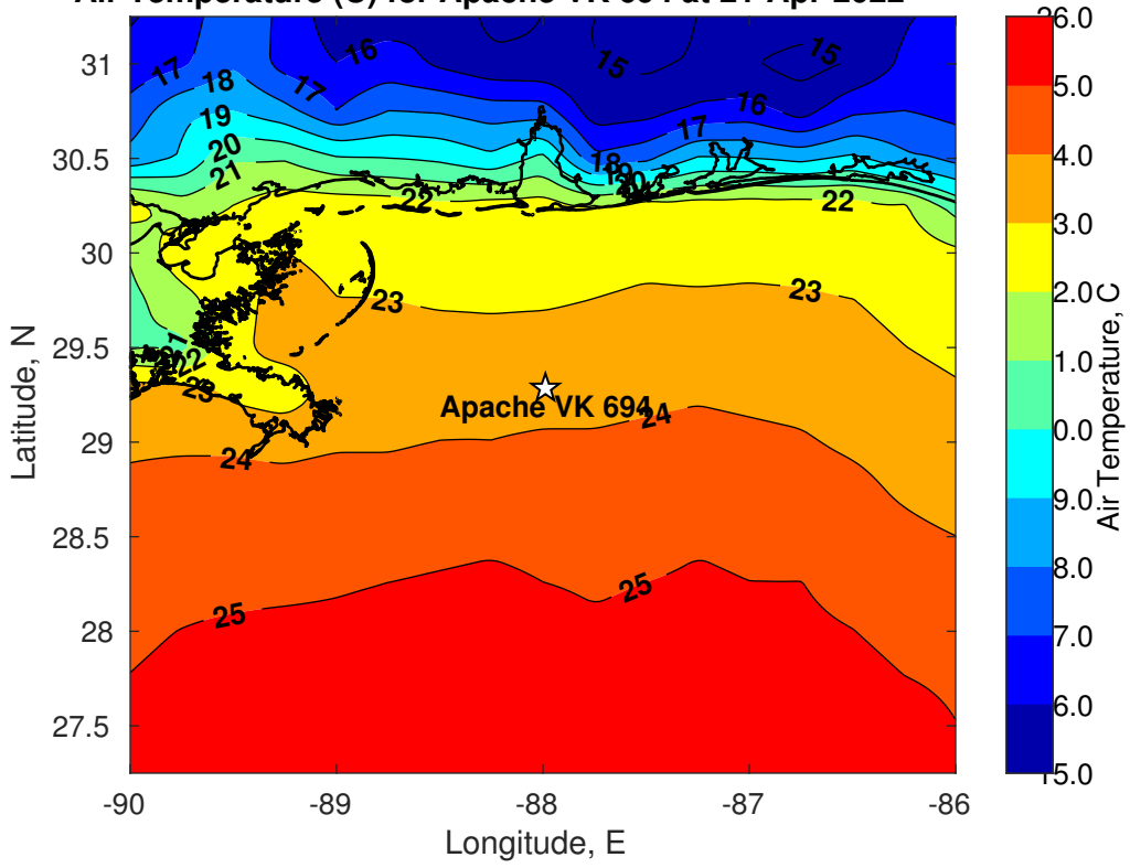
Air Temperature (C) for Apache VK 694 at 21-Apr-2022
